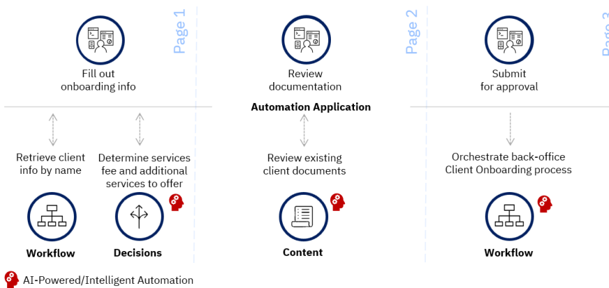
Figure 2: High-Level Client Onboarding Application Architecture
