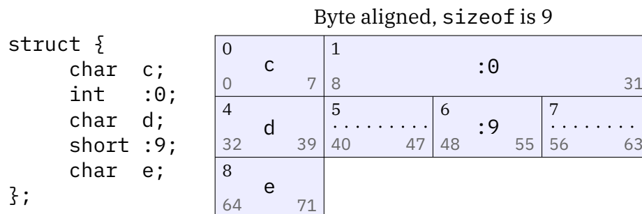
Figure 1.15.: Unnamed bit-fields
