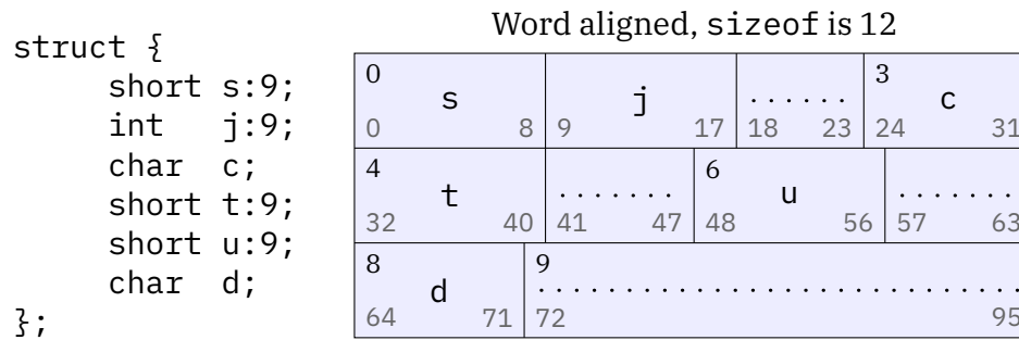
Figure 1.12.: Boundary alignment
