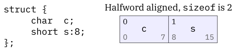
Figure 1.13.: Storage unit sharing
