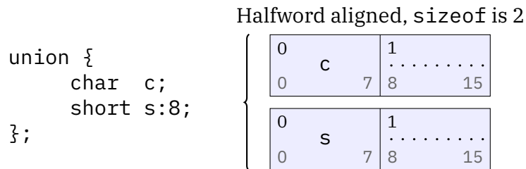
Figure 1.14.: Union allocation
