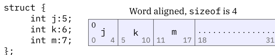
Figure 1.11.: Left-to-right allocation
