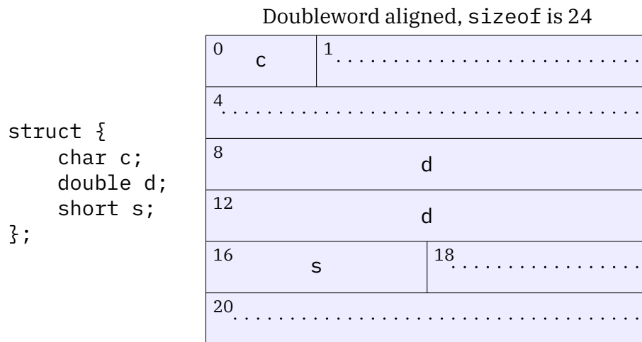
Figure 1.8.: Internal and tail padding
